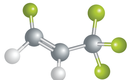
HFO-1234ze(Z)
