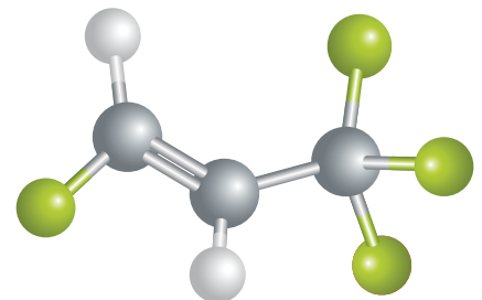
HFO-1234ze(E)
